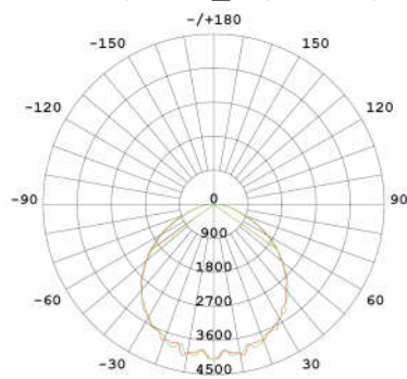
100W/UGR<22/112LM/W
